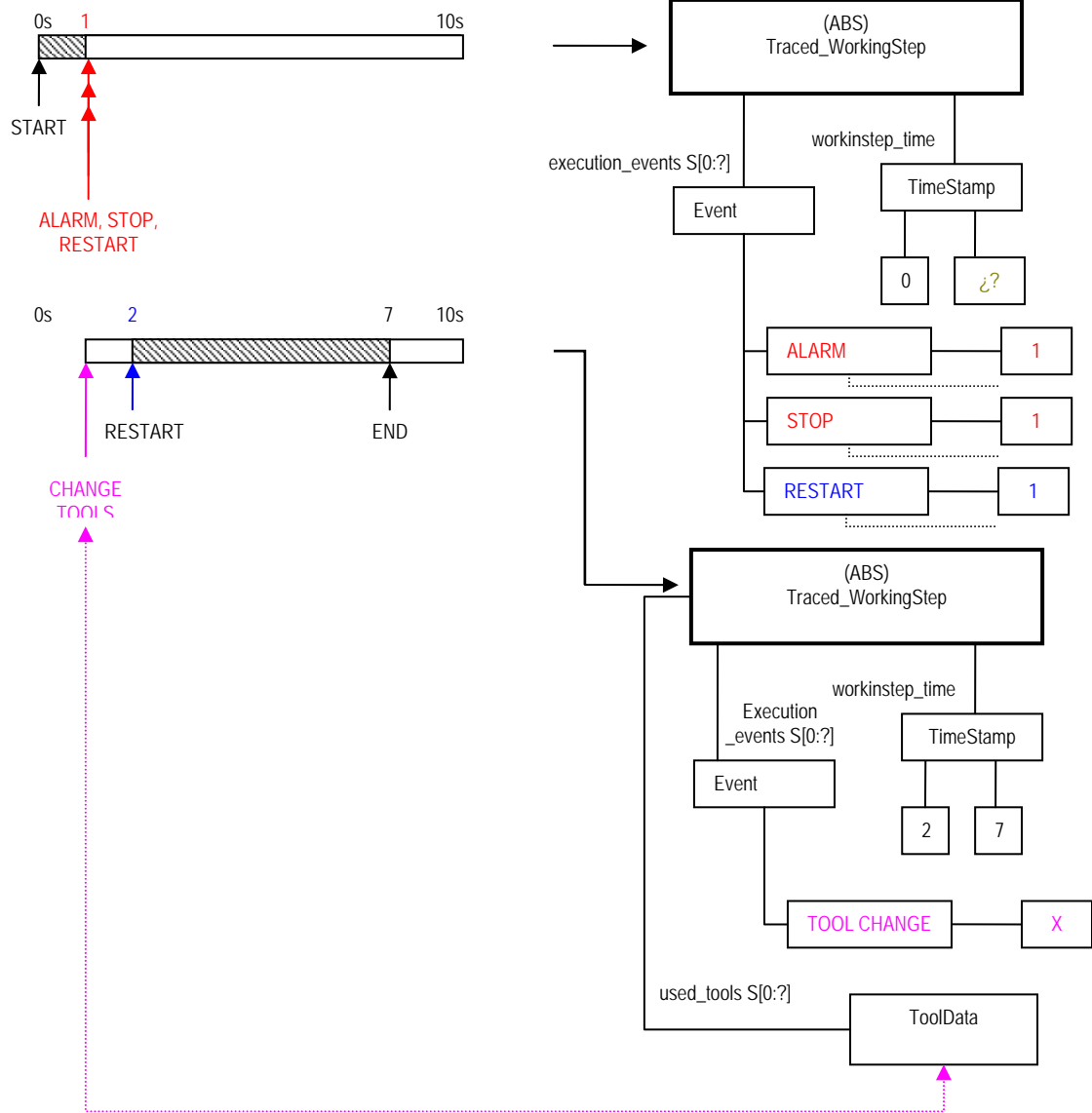
Figure 10. Controller events.
