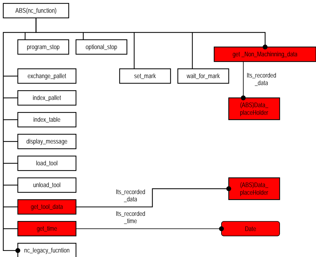
Figure 8. Some Identified Actions to perform by a NC TRACEABILITY-enabled machine. (non-axis movement operations)
