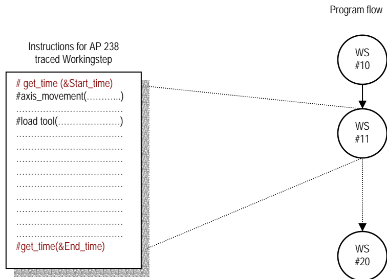
Figure 7. Getting Workinstep Execution Time.
