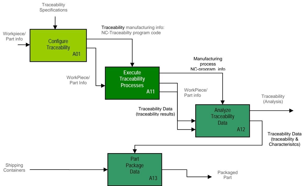
Adding capabilities to the Activity Model detail. (Preliminary)
