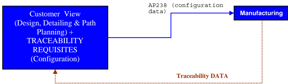
Framework for traceability application in STEP-NC.
