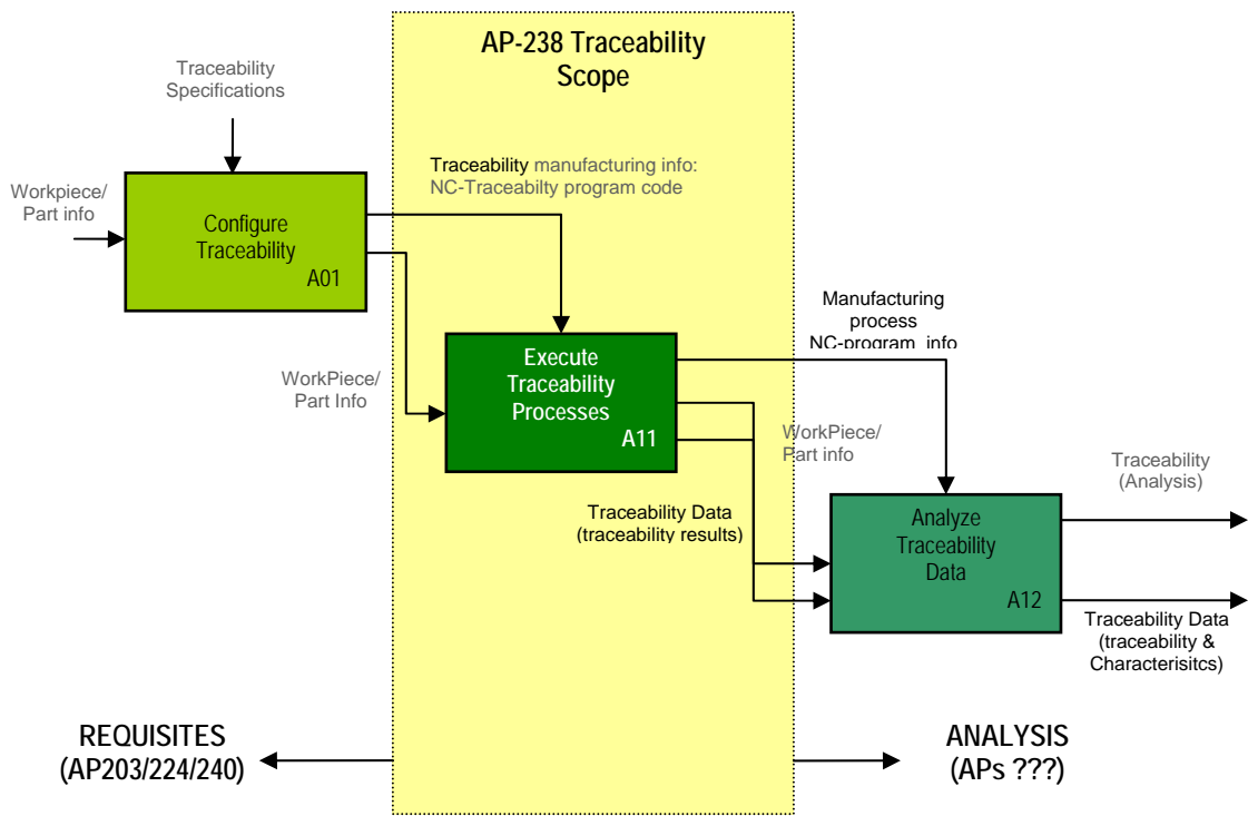
Activity Model detail. (Preliminary)
